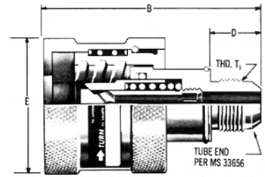
Coupling Half, Hydraulic Hose Attaching
