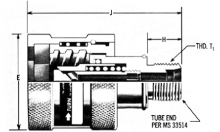
Coupling Half, Hydraulic Hose Attaching
