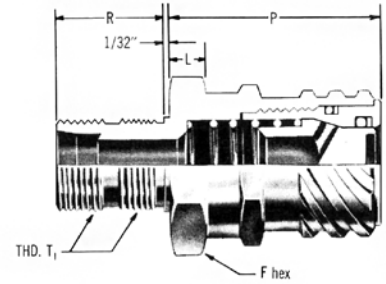
Coupling Half, Hydraulic Bulkhead Mounting
