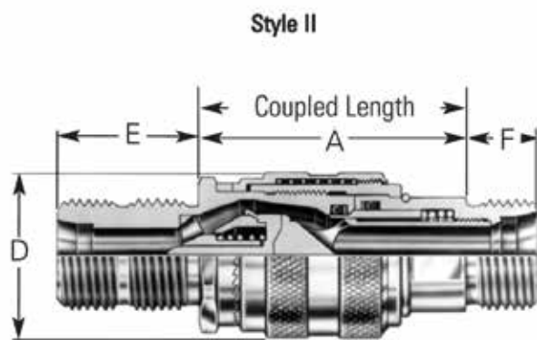
Coupling Half, Hose Attaching
